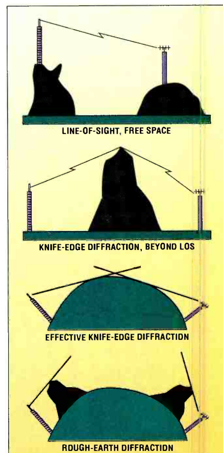
Figure 1. Graphic descriptions of four propagation modes.
