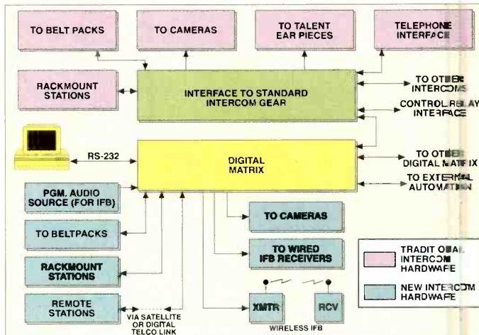
Figure 1. Block diagram of a fully featured current intercom system incorporating traditional equipment and new digital systems.
